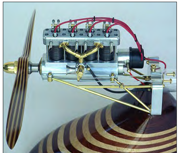
All his models are working engines, 4 cycle, hit & miss engines, all with hand made spark plugs.
